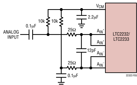
Figure 5. Single-Ended Drive
