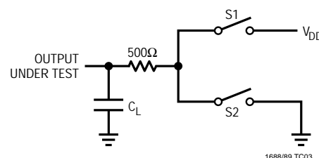
Figure 3. Driver Timing Test Load
