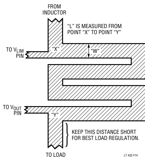
Figure 14. PCB trace Current Limit Sense Resistor with Kelvin Contacts
