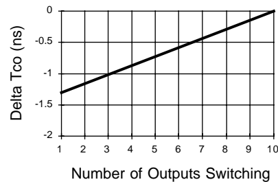
Delta Tco vs # of Outputs Switching
