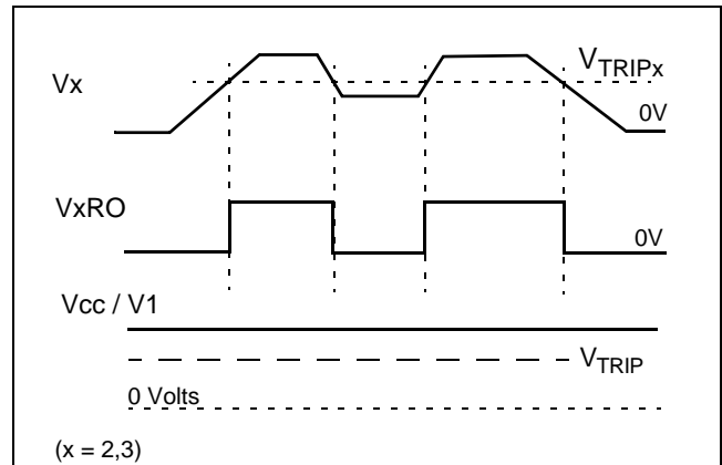
Figure 14. Voltage Monitor Response
