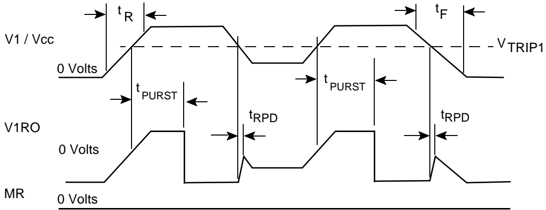
Figure 31. Manual Reset Timing Diagram
