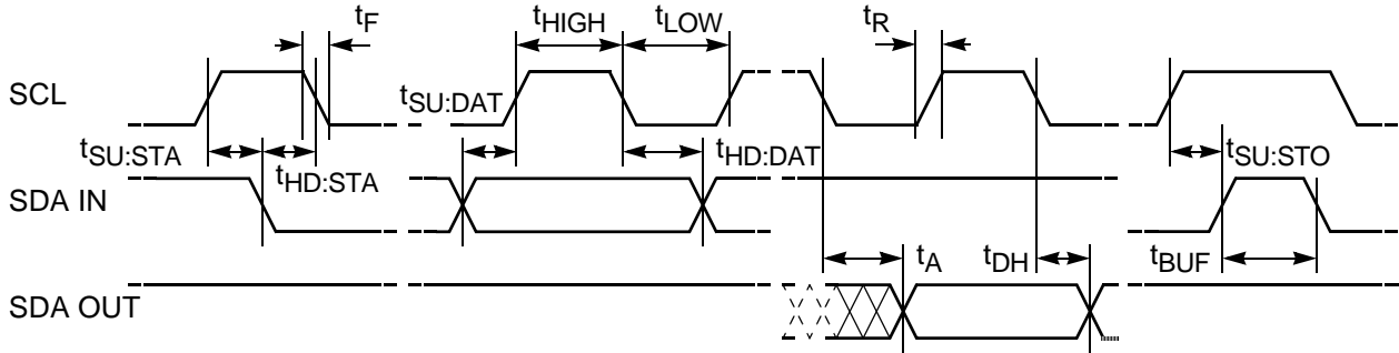
Figure 27. Bus Timing
