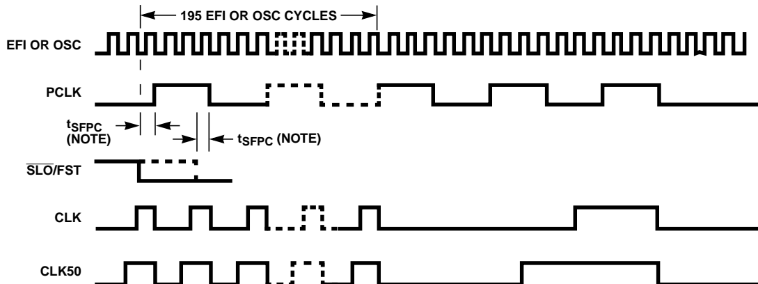
FIGURE 10. FAST TO SLOW CLOCK MODE TRANSITION
