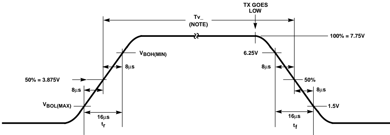
FIGURE 5. J1850 BUS WAVEFORM
