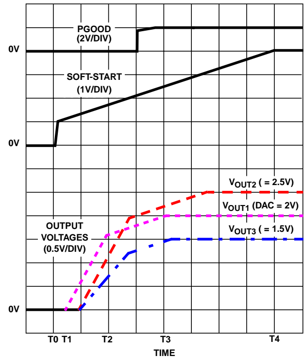
FIGURE 6. SOFT-START INTERVAL
