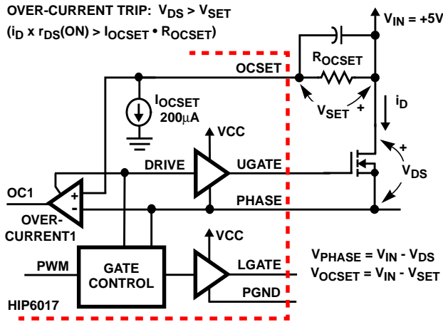
FIGURE 9. OVER-CURRENT DETECTION
