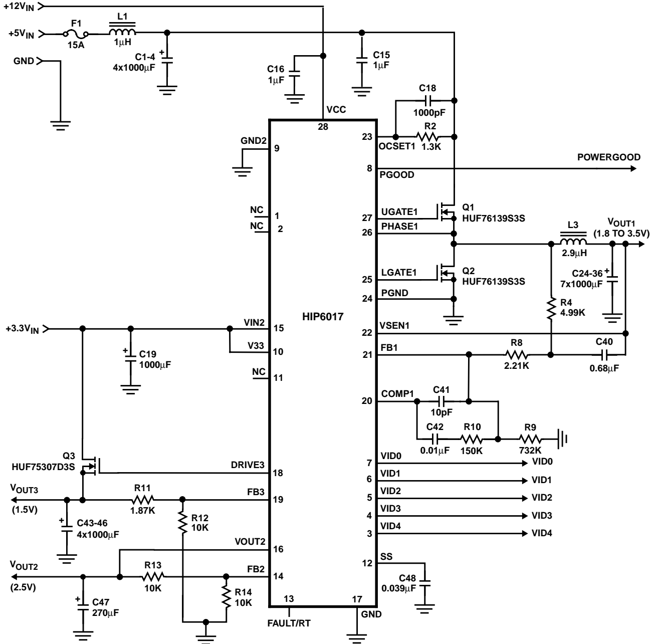
FIGURE 15. APPLICATION CIRCUIT
