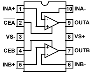
EL5252 (10-PIN MSOP) TOP VIEW
