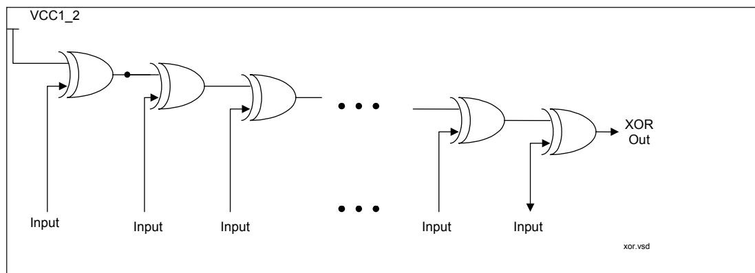
Figure 9. XOR–Tree Chain
