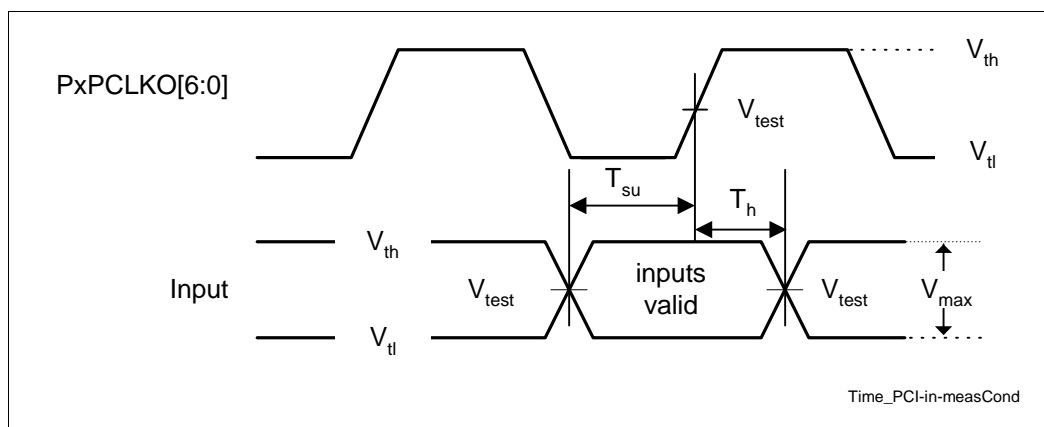
Figure 17. PCI Input Timing
