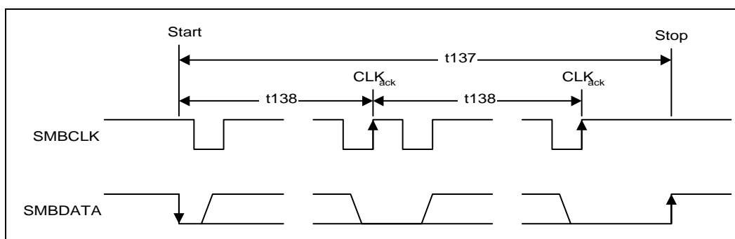
Figure 16-17. SMBus Timeout
