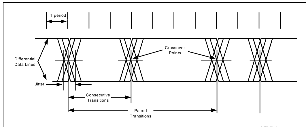
Figure 16-14. USB Jitter
