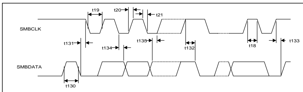
Figure 16-17. SMBus Timeout
