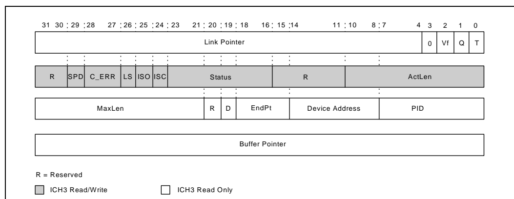
Figure 5-15. Transfer Descriptor
