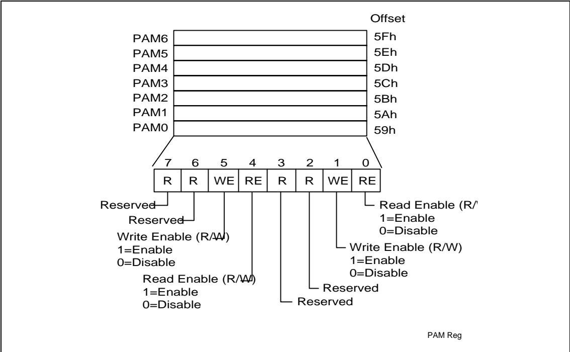
Figure 3. PAM Registers
