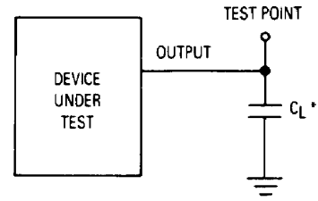
*Includes all probe and jig capacitance.
