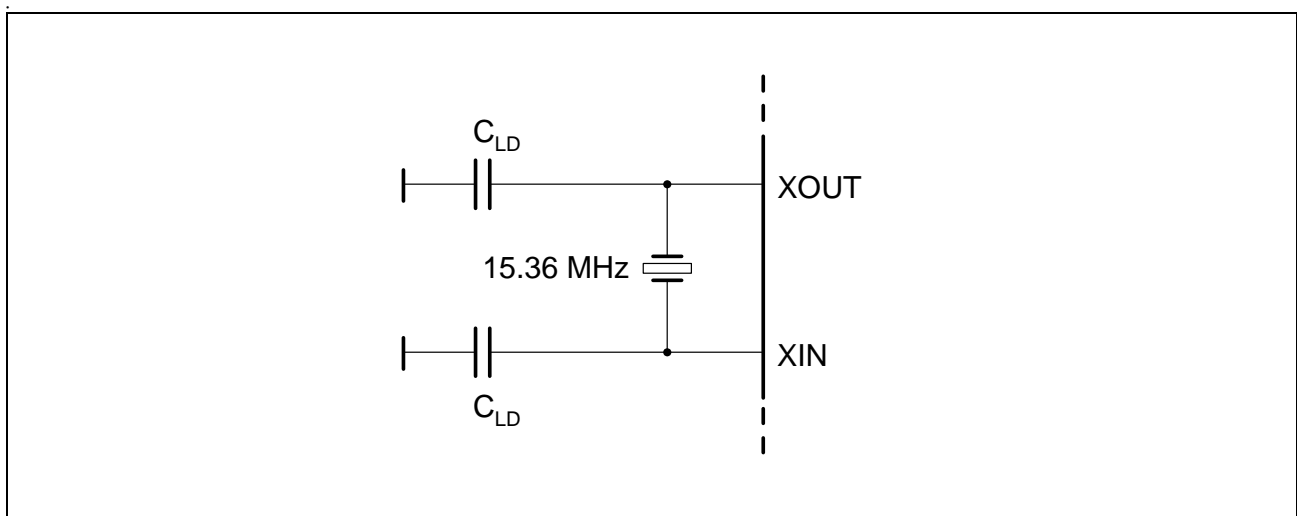
Figure 71 Crystal Oscillator
