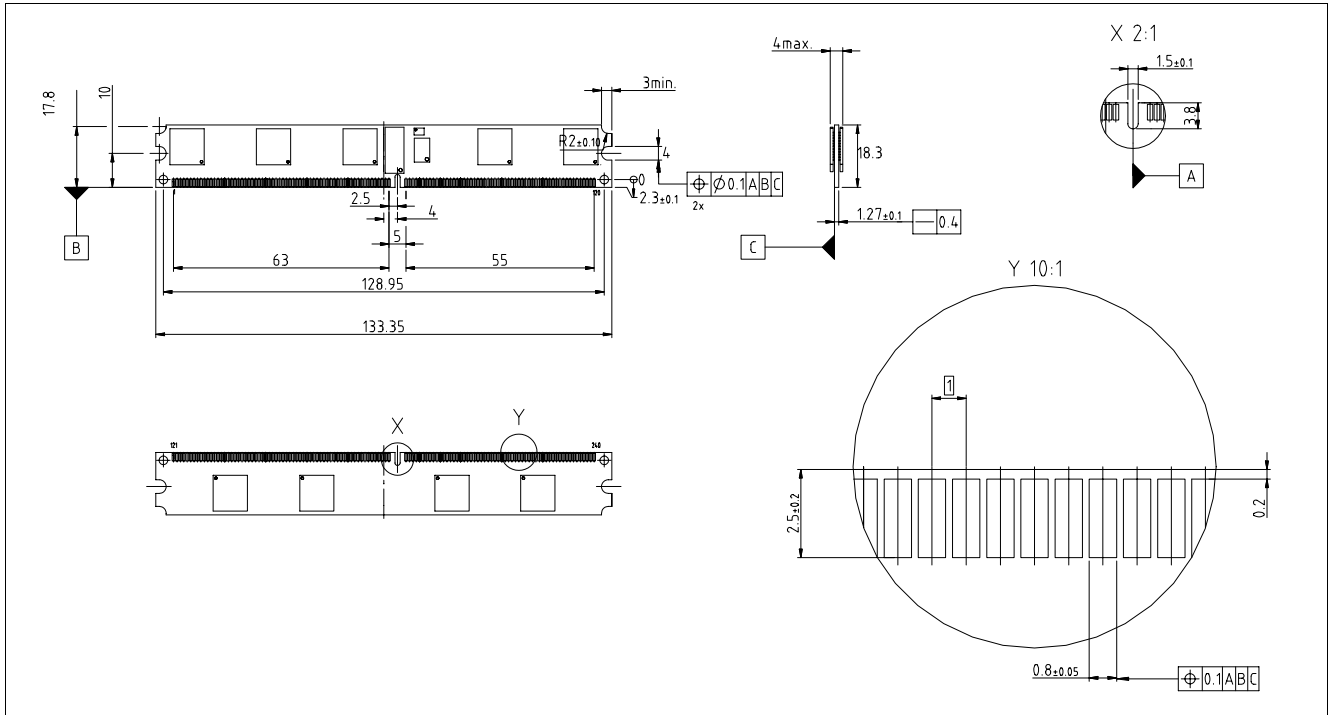
Figure 5 Package Outline Raw Card R L-DIM-240-51
