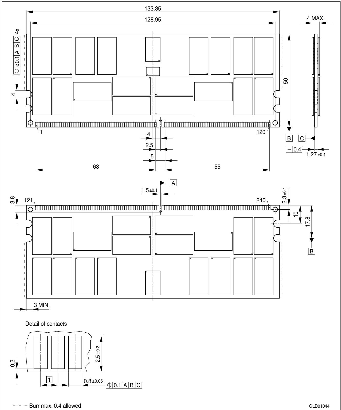
Figure 3 Package Outline Raw Card ZZ - L-DIM-240-42
