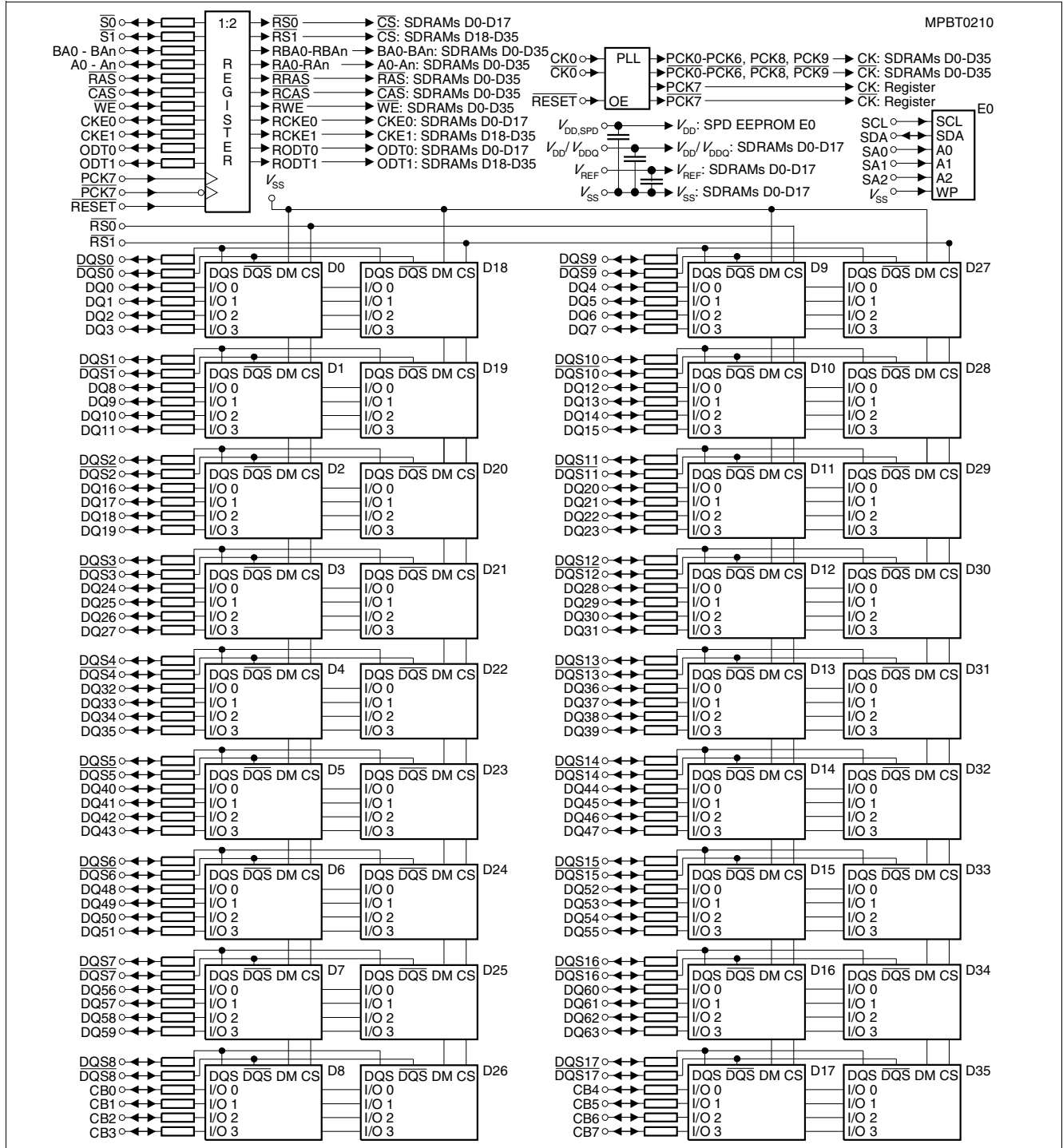
Figure 2 Block Diagram Raw Card ZZ RDIMM (x72, 2Ranks, x4)
