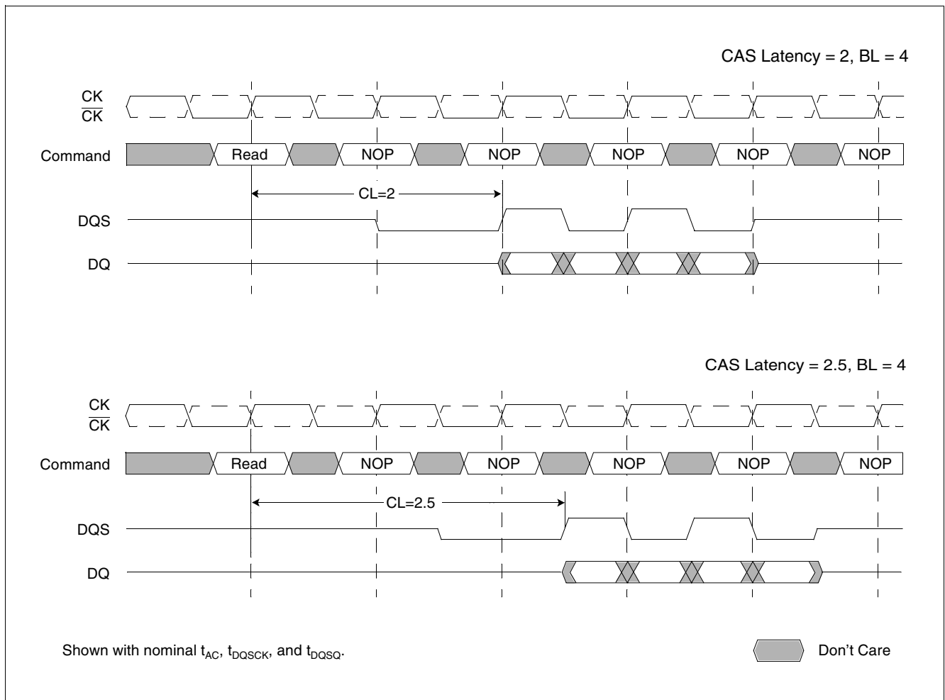
Figure 5 Required CAS Latencies
