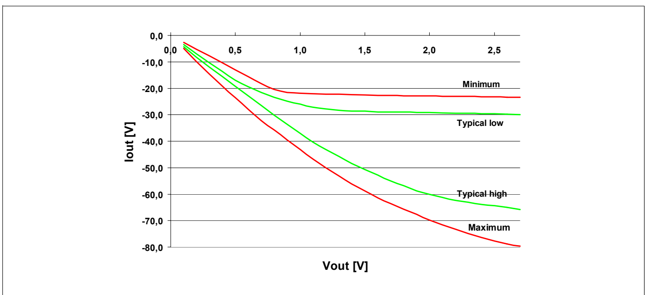
Figure 35 Weak Strength Pull-up Characteristics
