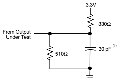
LOAD CIRCUIT
