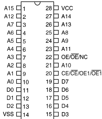
HT23C512 - 28 DIP/SOP
