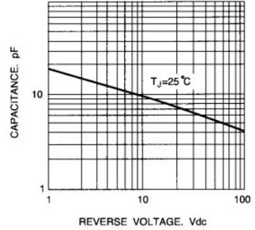
Fig. 2 - TYPICAL JUNCTION CAPACITANCE
