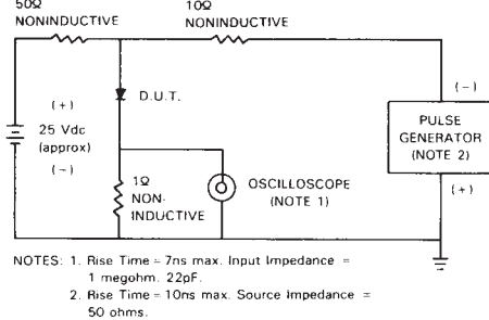
FIG. 3 - TYPICAL REVERSE CHARACTERISTICS
