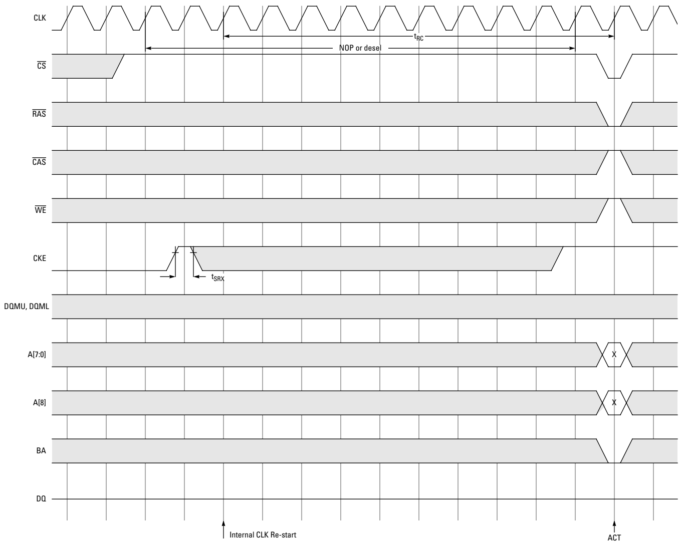
Figure 36. Self-Refresh Exit
