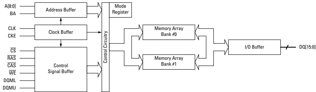
Figure 1. 4M (2-Bank x 131072-Word x 16-Bit) Synchronous DRAM
