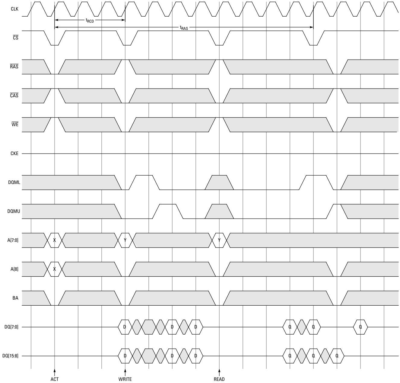
Figure 29. DQM Byte Control for WRITE 3030to READ (Single Bank) BL=4, CL=3
