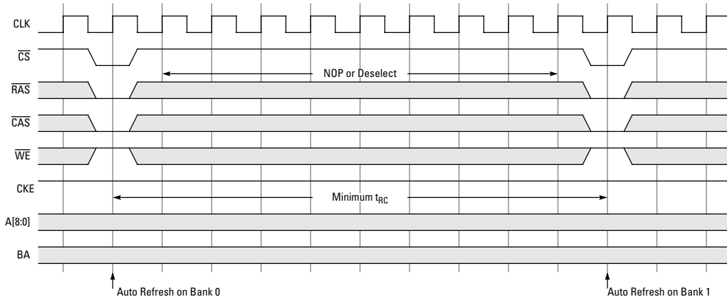
Figure 17. Auto Refresh
