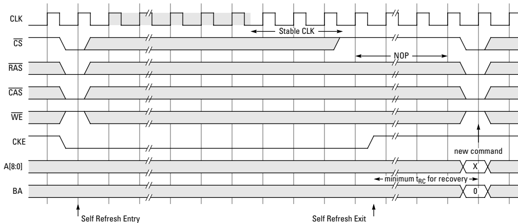
Figure 18. Self-Refresh
