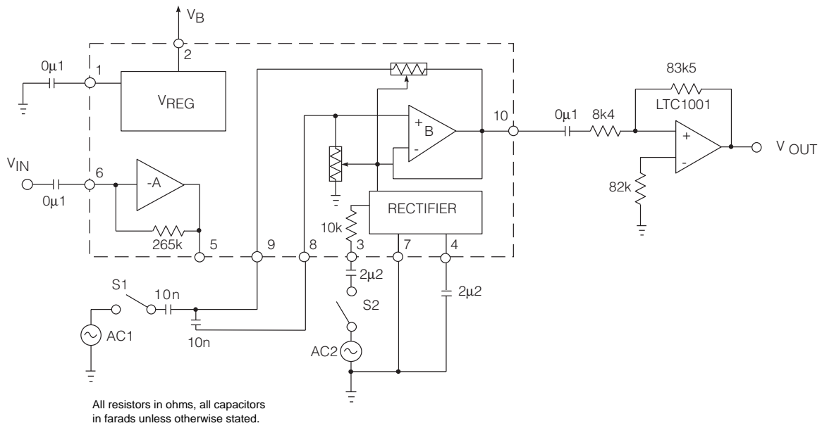
Fig. 1 Test Circuit
