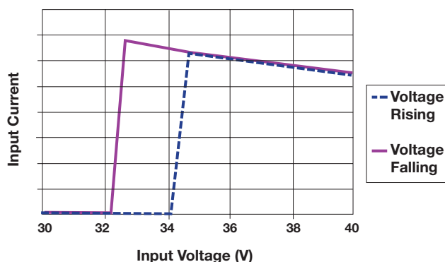
Undervoltage Lockout
