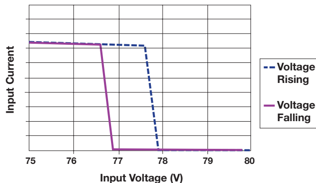
Overvoltage Lockout
