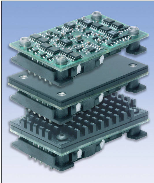
The open-frame Pisces is available with an optional baseplate or low profile heatsink for maximum thermal performance.
