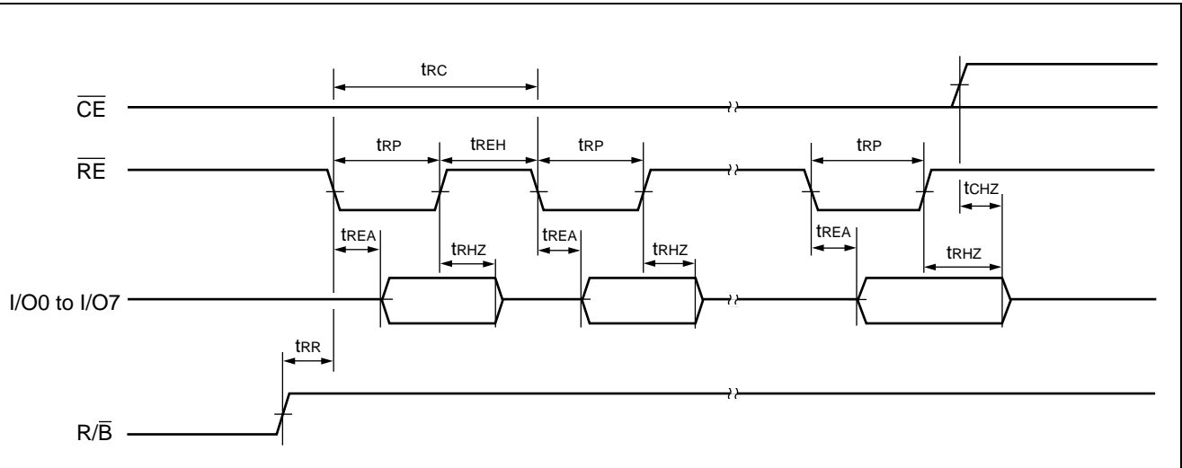
Figure 12 Serial Read Cycle Timing Diagram
