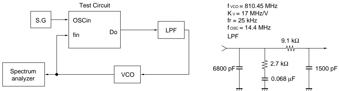
PLL phase noise
