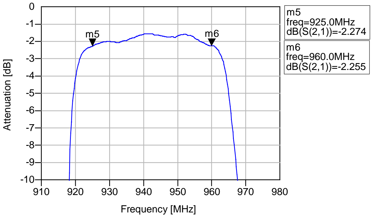
Fig.3 In-band Characteristics
