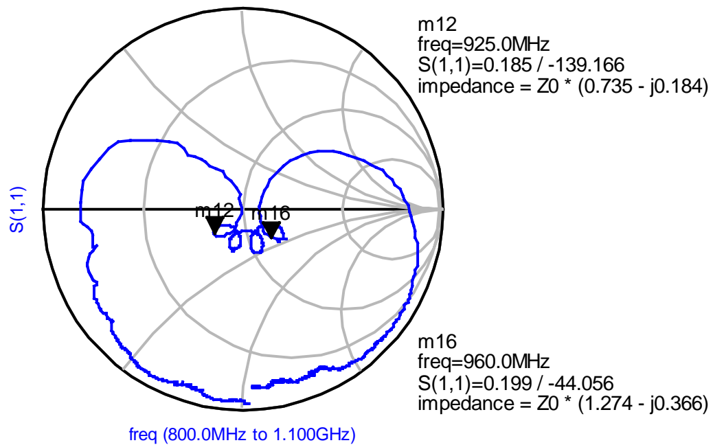
Fig.5 S11
