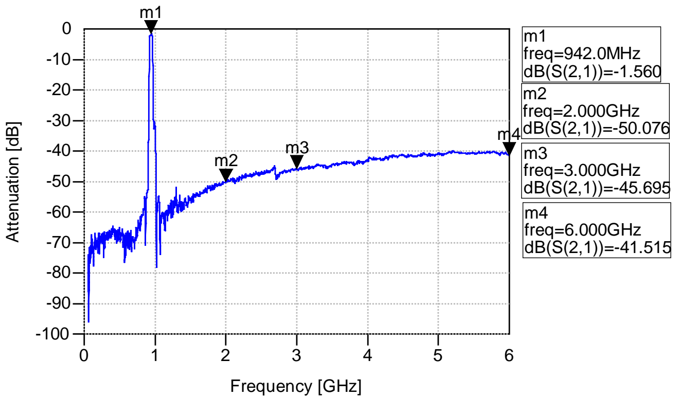
Fig.4 Wide-band Characteristics
