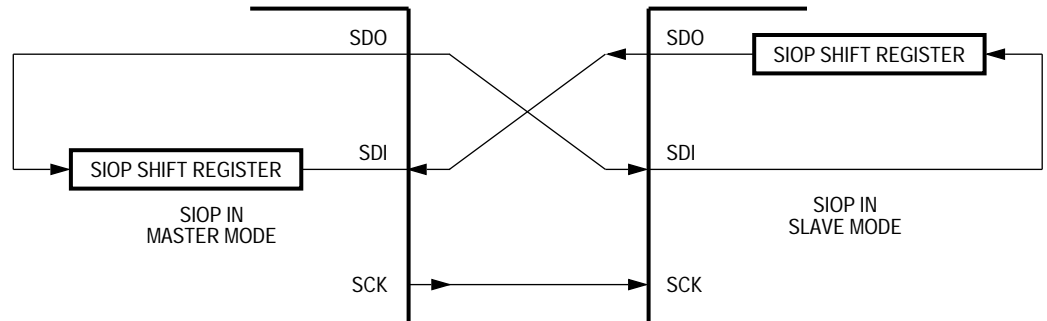
Figure 62. Master/Slave SIOPI Shift Register Operation
