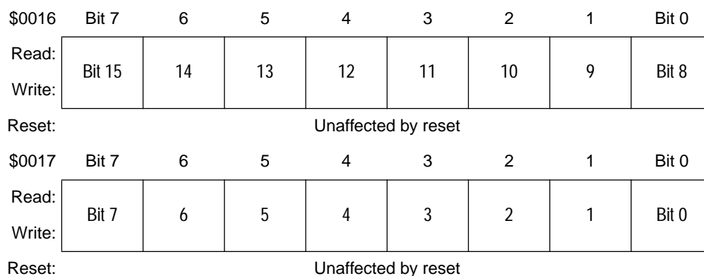
Figure 58. Output Compare Registers (OCRH and OCRL)
