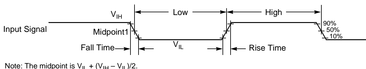
Figure 10-1 Input Signal Measurement References
