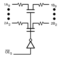
4-Bit Configuration
