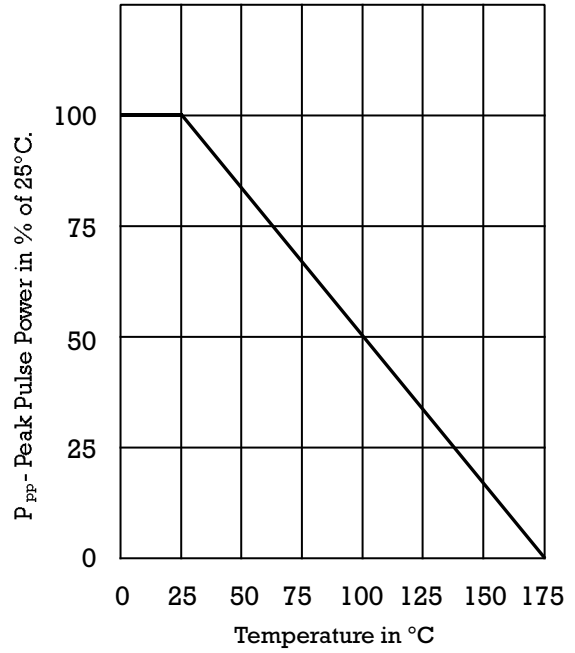
DERATING CURVE
