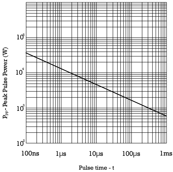
PEAK PULSE POWER RATING CURVE
