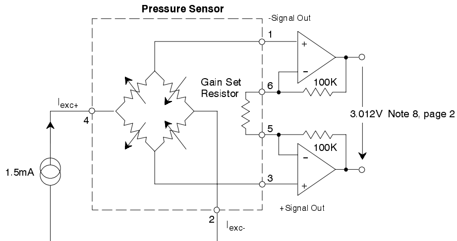
Figure 1. SM5611 and SM5651 with Constant Current Supply and Differential Output
