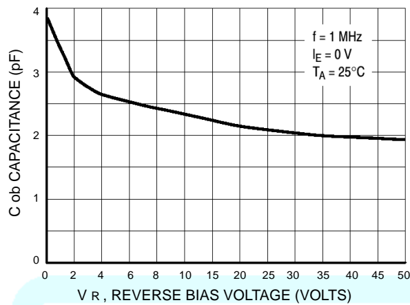
Figure 34. Output Capacitance
