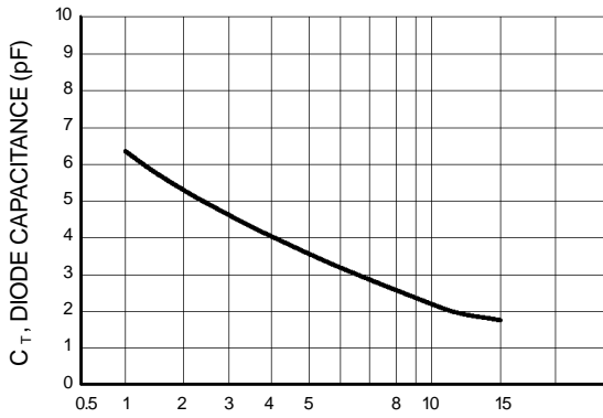
V R , REVERSE VOLTAGE (VOLTS) Figure 1. Diode Capacitance
