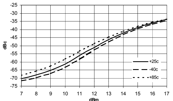
IS-95 @ 1950MHz Adj. Channel Pwr. Vs. Channel Output Pwr.
