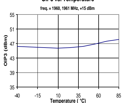
OIP3 vs. Temperature
