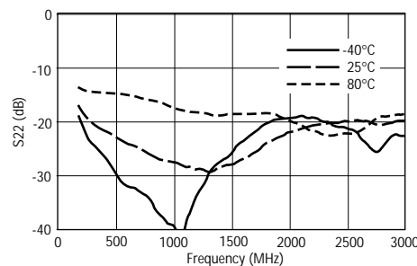
S22 vs. Frequency over Temperature
