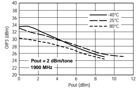
OIP3 vs. Pout over Temperature
