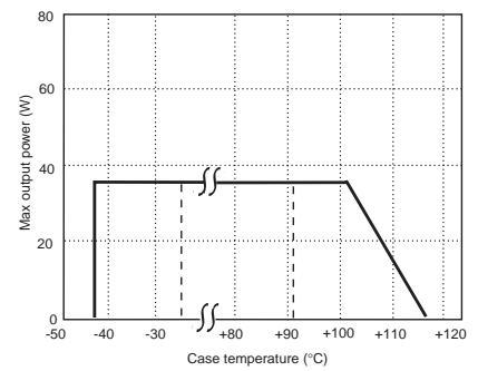
Power derating
