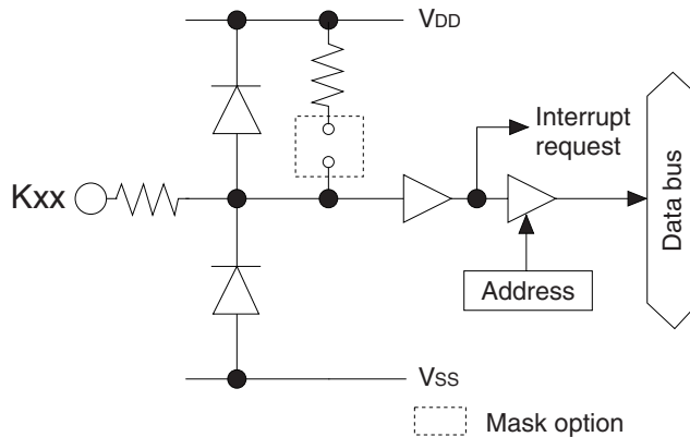
Fig. 4.4.1.1 Configuration of input port
