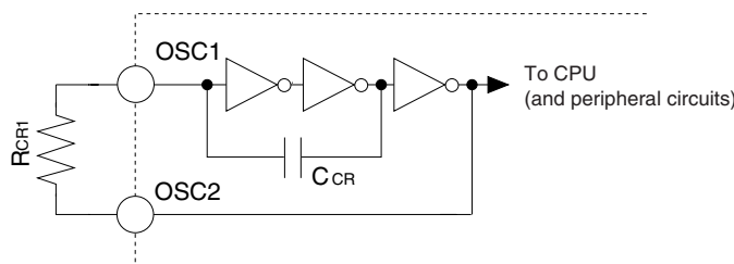
(b) CR oscillation circuit
