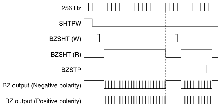
Fig. 4.12.6.1 Timing chart for one-shot output
