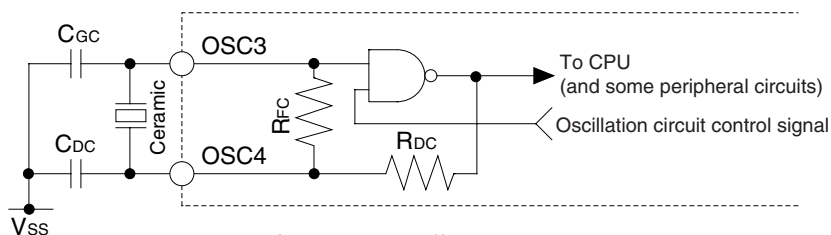
(b) Ceramic oscillation circuit
