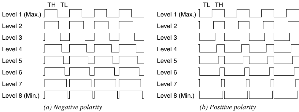
Fig. 4.12.4.1 Duty ratio of the buzzer signal waveform
