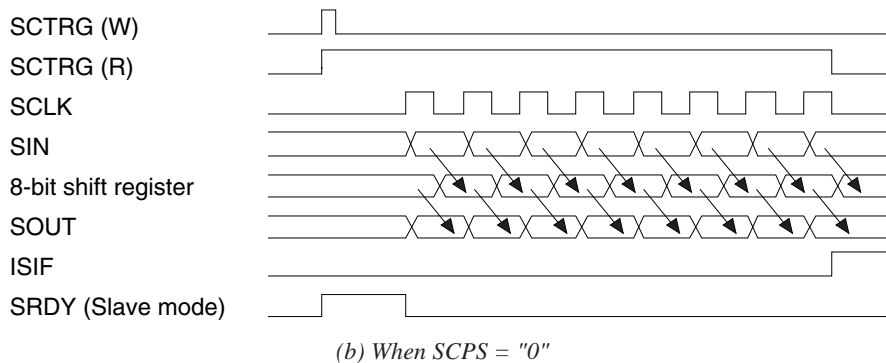
Fig. 4.11.4.3 Serial interface timing chart (when synchronous clock is positive polarity SCLK)
