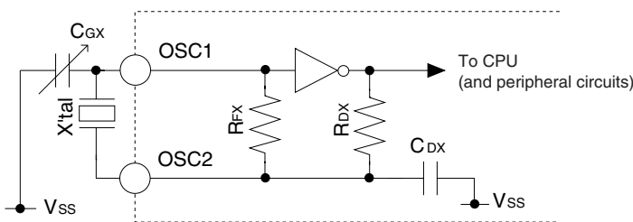
(a) Crystal oscillation circuit
