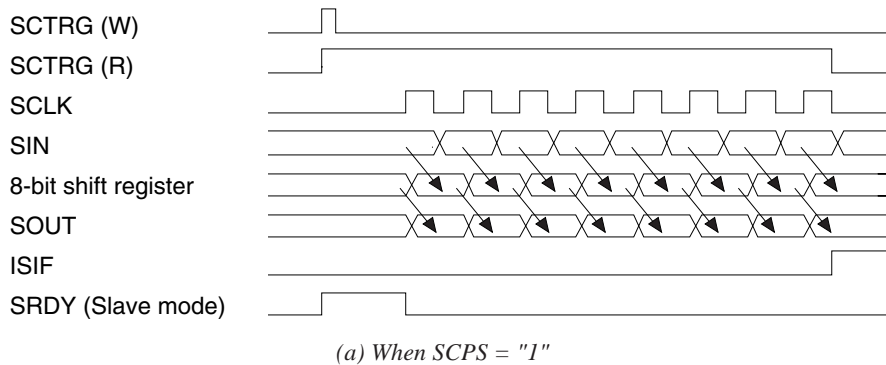
Fig. 4.11.4.2 Serial interface timing chart (when synchronous clock is negative polarity \overline{SCLK} )
