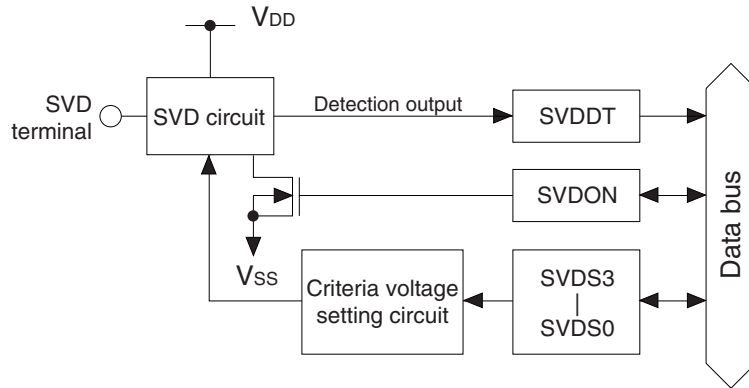
Fig. 4.13.1.1 Configuration of SVD circuit
