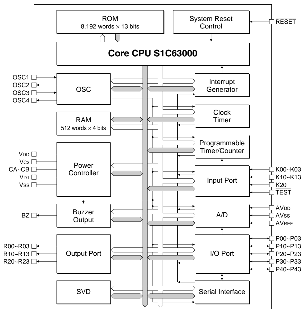
Fig. 1.2.1 Block diagram
