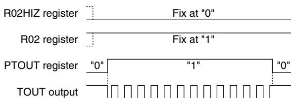
Fig. 4.10.3.5.2 Output waveform of the TOUT signal
