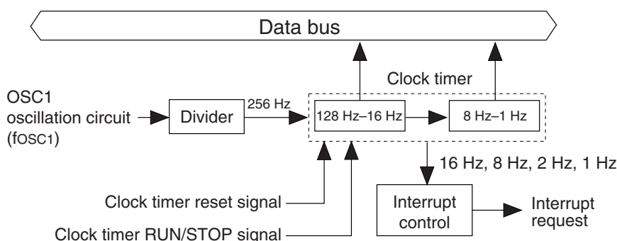
Fig. 4.8.1.1 Block diagram for the clock timer
