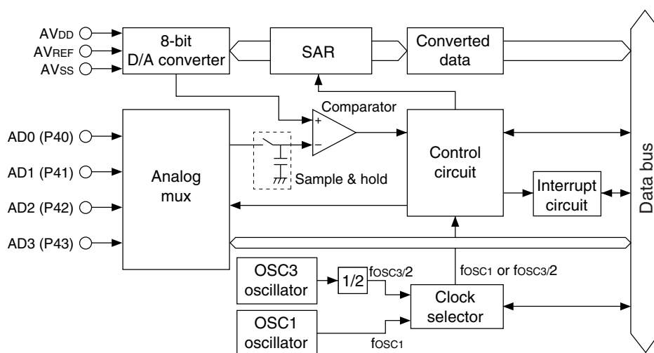
Fig. 4.9.1.1 Configuration of A/D converter
