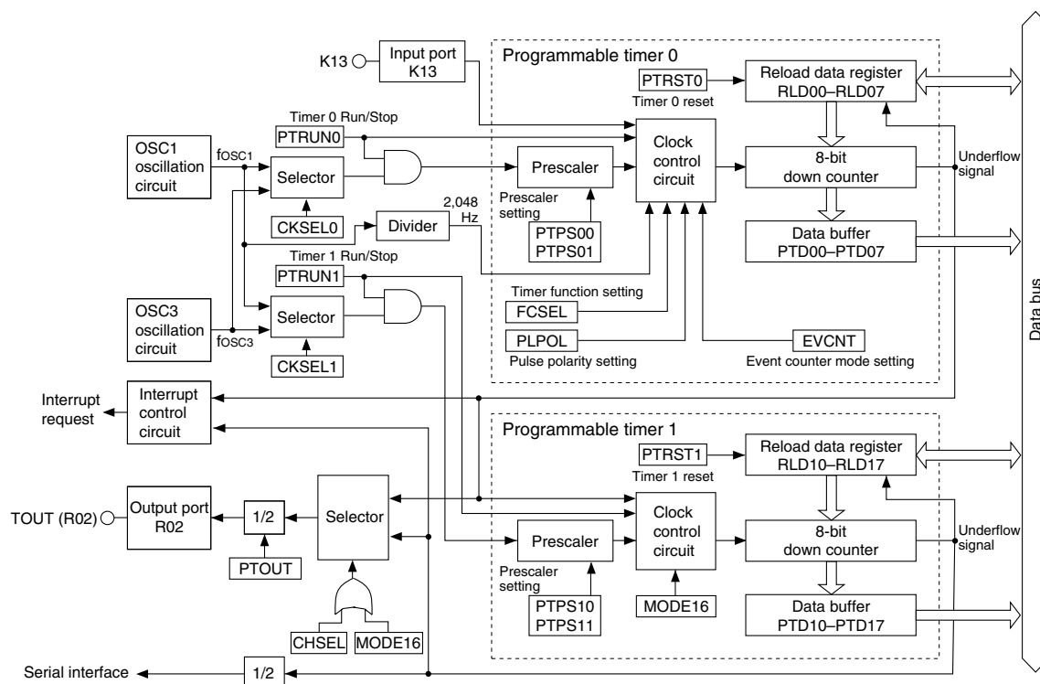
Fig. 4.10.1.1 Configuration of programmable timer
