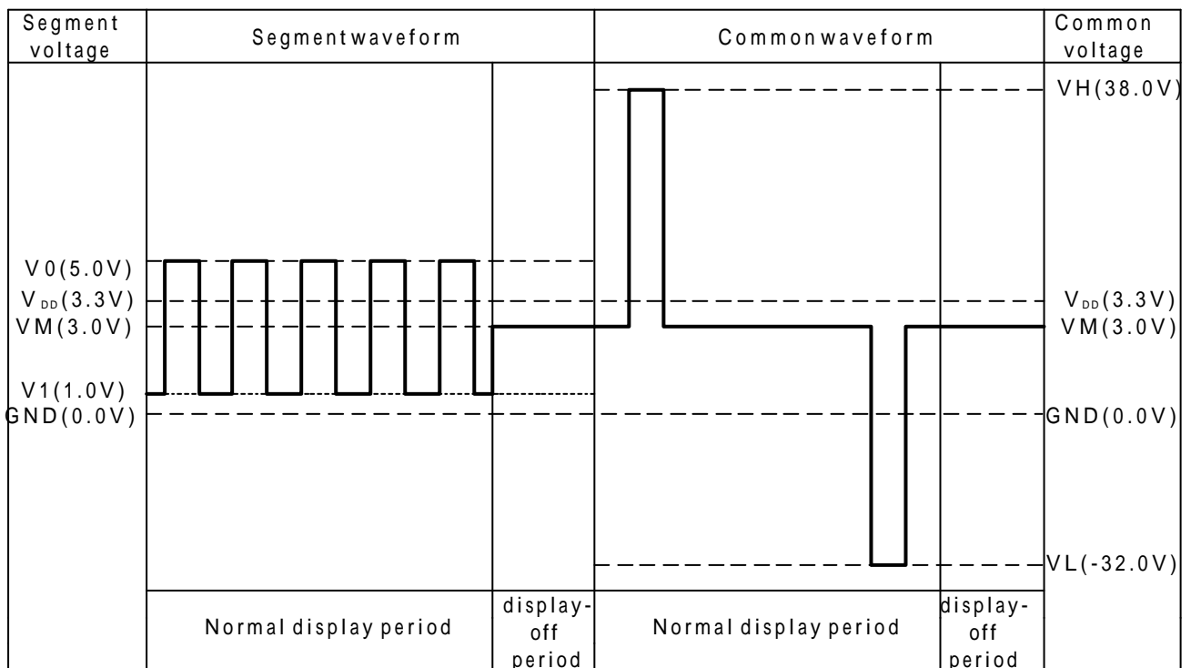
Figure 14. Signal voltage
