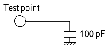
Figure 15. Load circuit for output delay time
