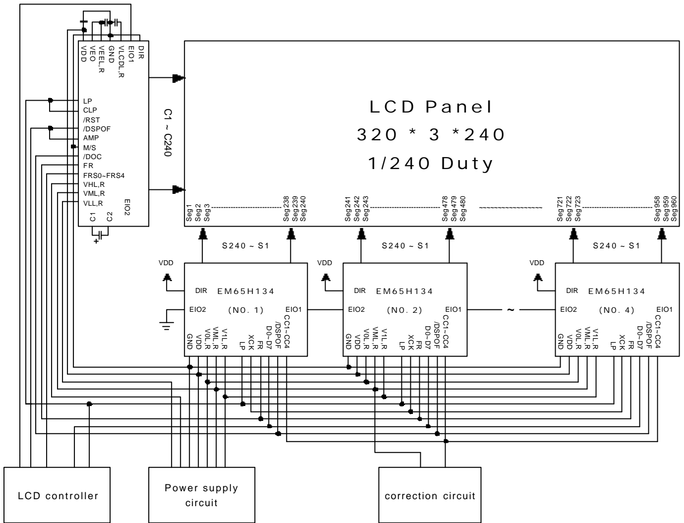
Figure 17. Application circuit
