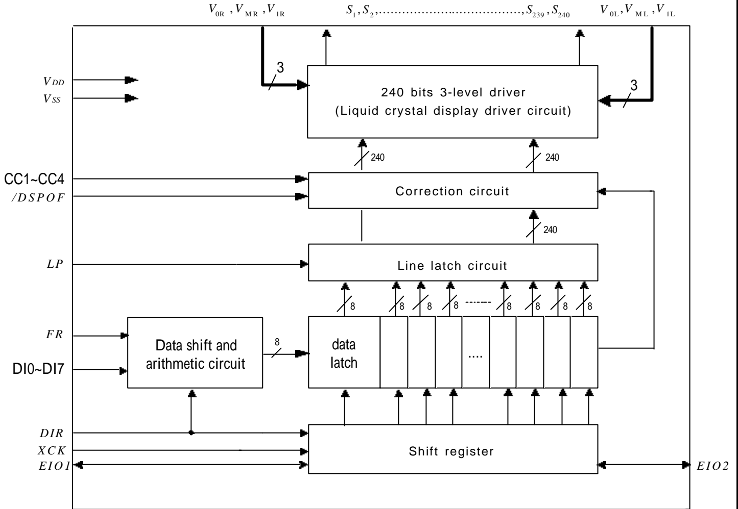
Figure 2. Block diagram
