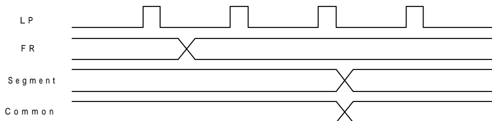
Figure 3. FR、LP、output timing
