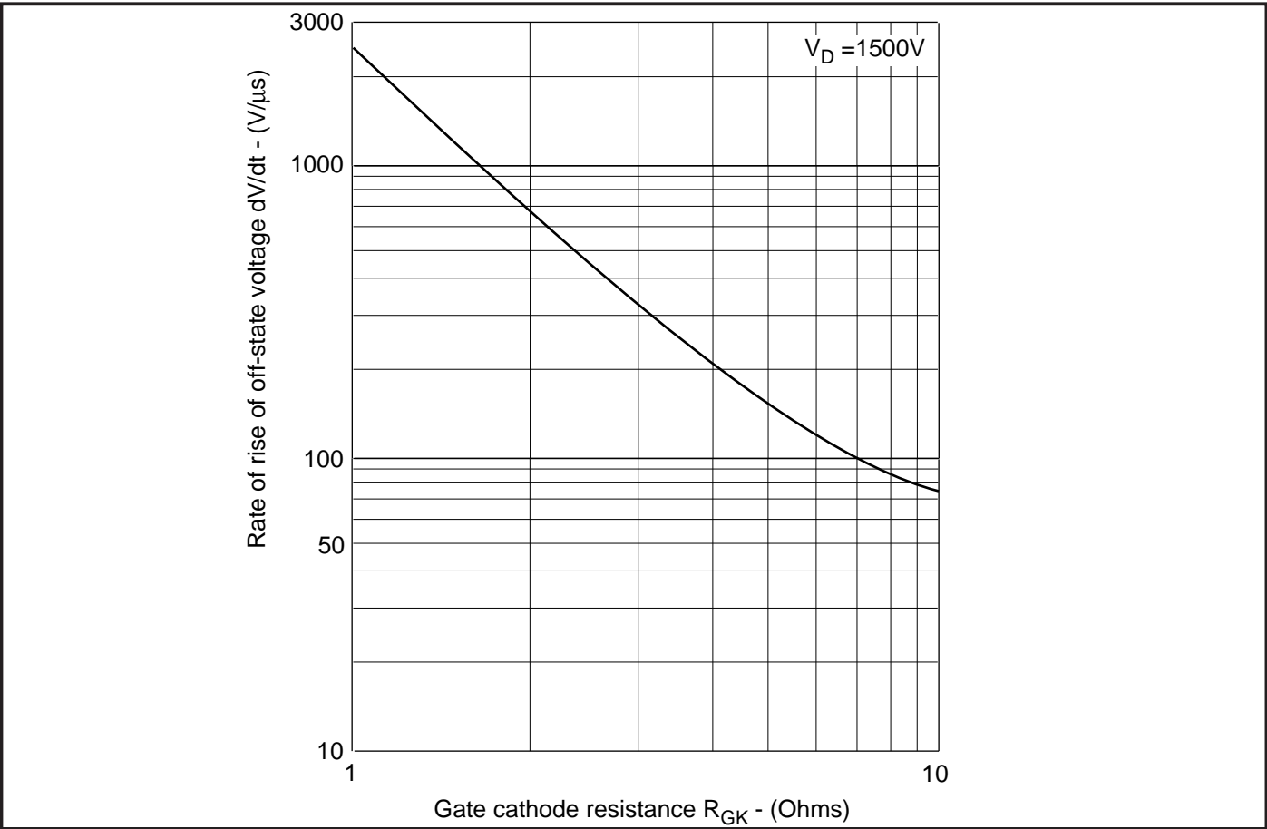
Fig.28 Typical rate of rise of off-state voltage vs gate cathode resistance
