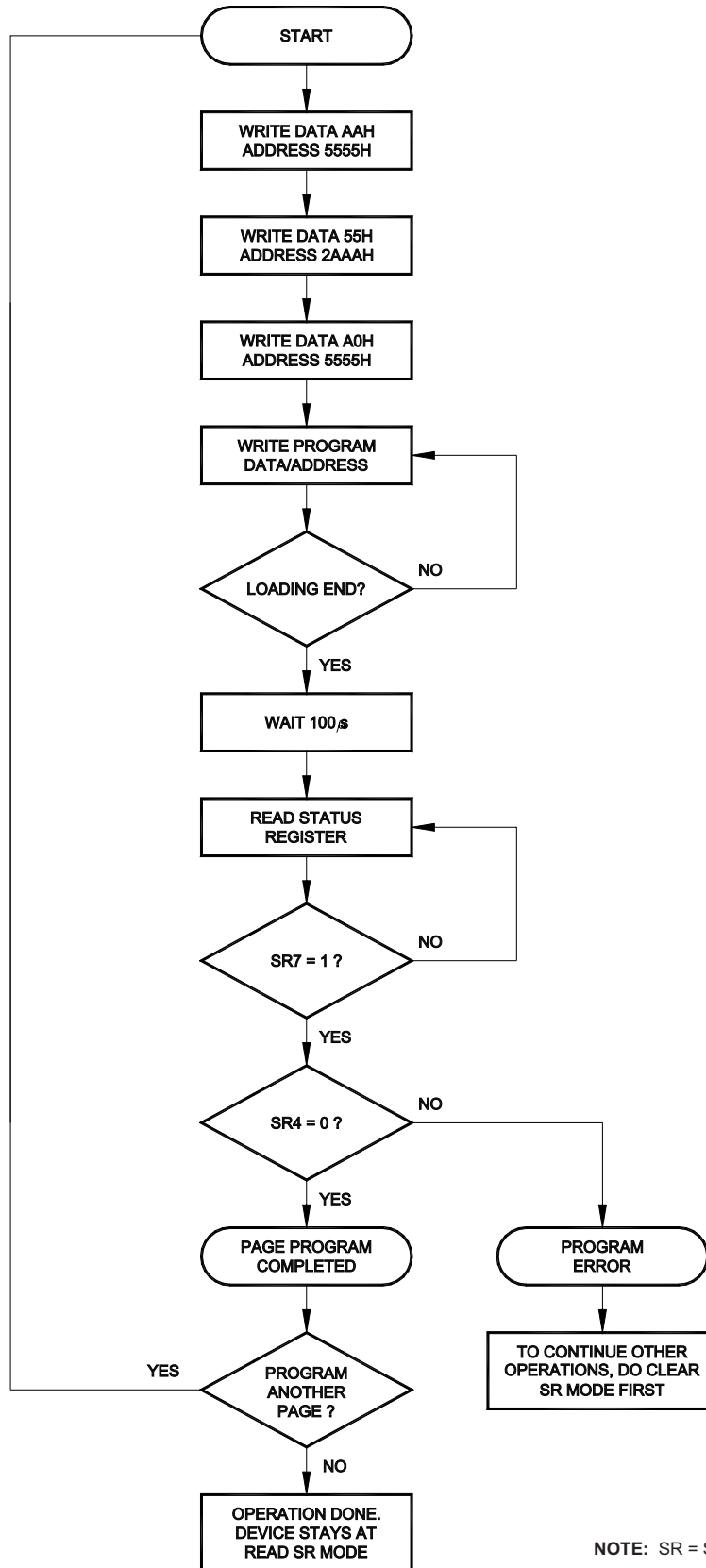
FIGURE 1: AUTOMATIC PAGE PROGRAM FLOW CHART 11
