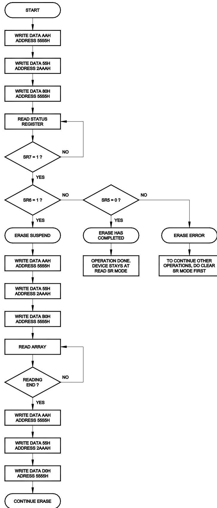
FIGURE 4: ERASE SUSPEND/ERASE RESUME FLOW CHART 11
