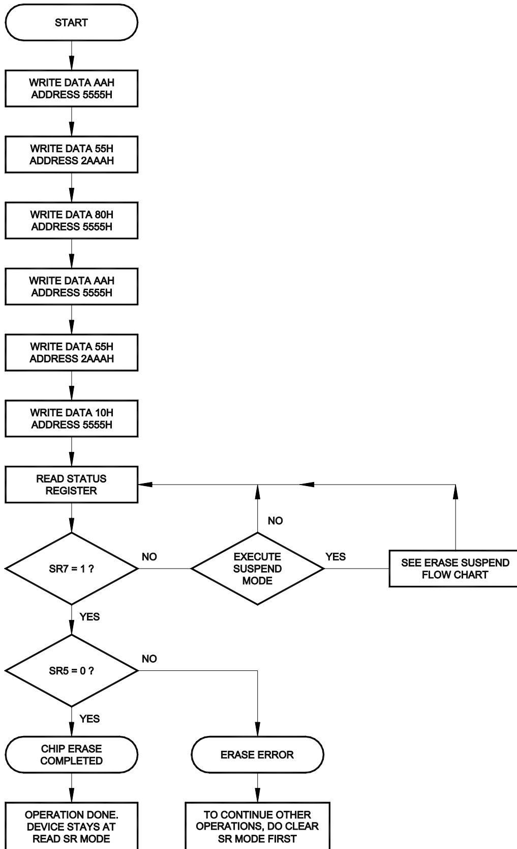
FIGURE 2: AUTOMATIC CHIP ERASE FLOW CHART 11
