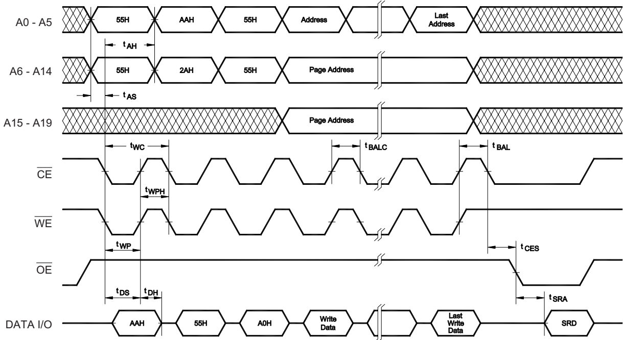
Figure 7: AUTOMATIC PAGE PROGRAM CYCLE 10
