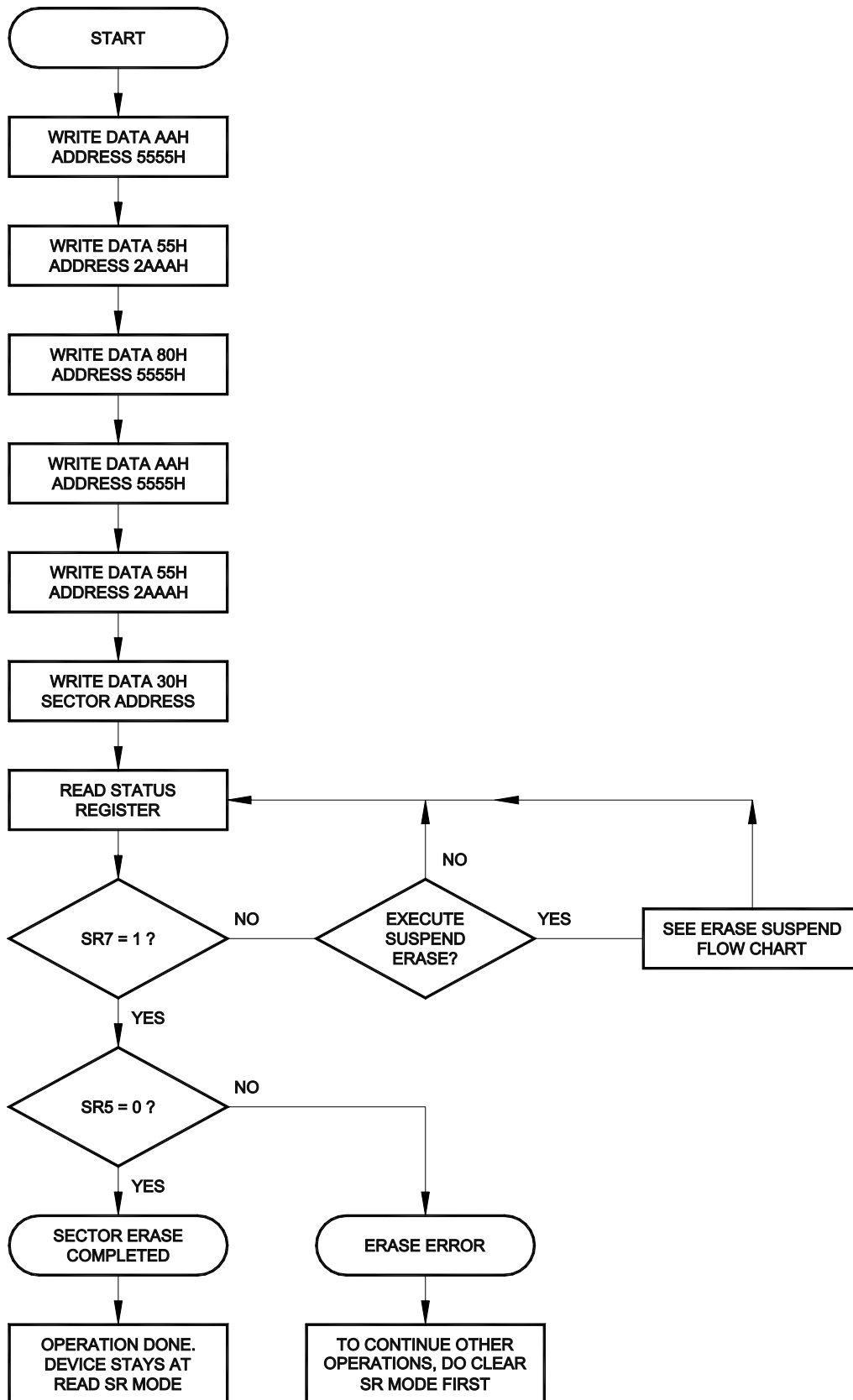
FIGURE 3: AUTOMATIC SECTOR ERASE FLOW CHART 11
