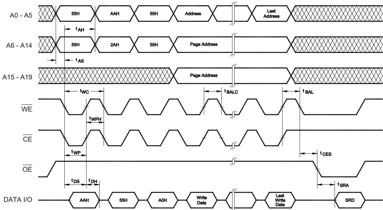
Figure 10: AUTOMATIC PAGE PROGRAM TIMING CYCLE 10
