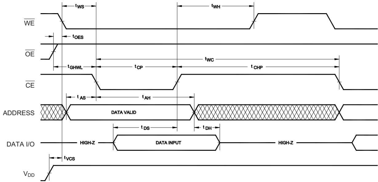
Figure 9: COMMAND WRITE CYCLE (Alternate \overline{CE} Controlled)
