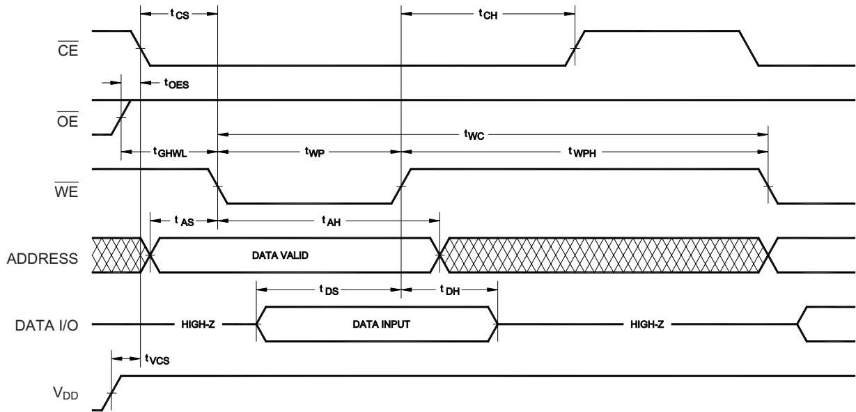
Figure 6: WRITE CYCLE
