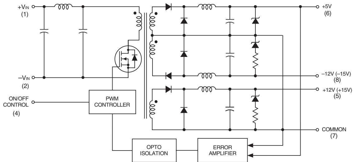
Figure 1. Simplified Schematic
