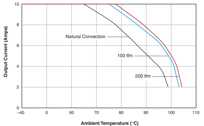
LSN-2.5/10-D3 Output Current vs. Ambient Temperature (Vertical mount, air flow direction from pin 1 to pin 11)
