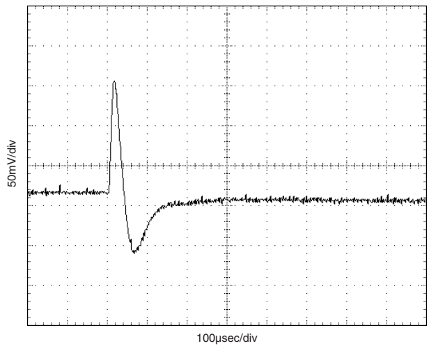
Dynamic Load Response (VIN = 3.3V, VOUT = 2.5V, 100% to 0% Load Step, No External COUT)
