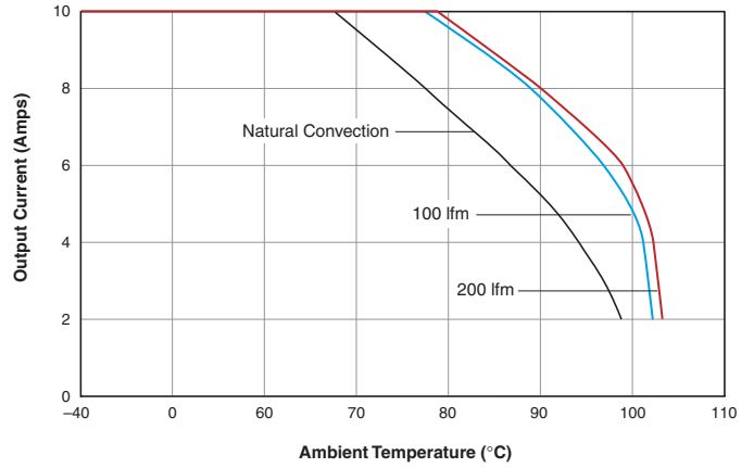
LSN-1.5/10-D3 Output Current vs. Ambient Temperature (Vertical mount, air flow direction from pin 1 to pin 11)
