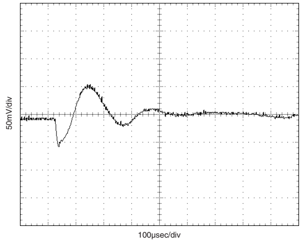
Dynamic Load Response (VIN = 3.3V, VOUT = 2.5V, 0% to 100% Load Step, COUT = 5000µF OSCON)
