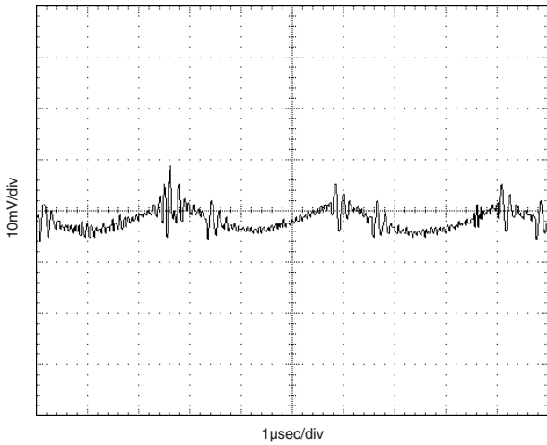
Output Ripple/Noise (VIN = 3.3V, VOUT = 2.5V, No Load, No External Capacitor)
