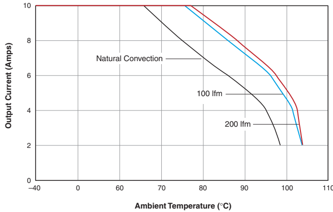
LSN-1.8/10-D3 & LSN-2/10-D3 Output Current vs. Ambient Temperature (Vertical mount, air flow direction from pin 1 to pin 11)
