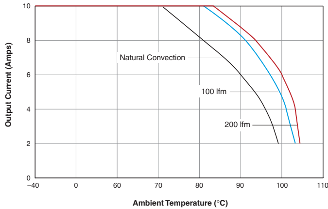
LSN-1/10-D3 & LSN-1.2/10-D3 Output Current vs. Ambient Temperature (Vertical mount, air flow direction from pin 1 to pin 11)
