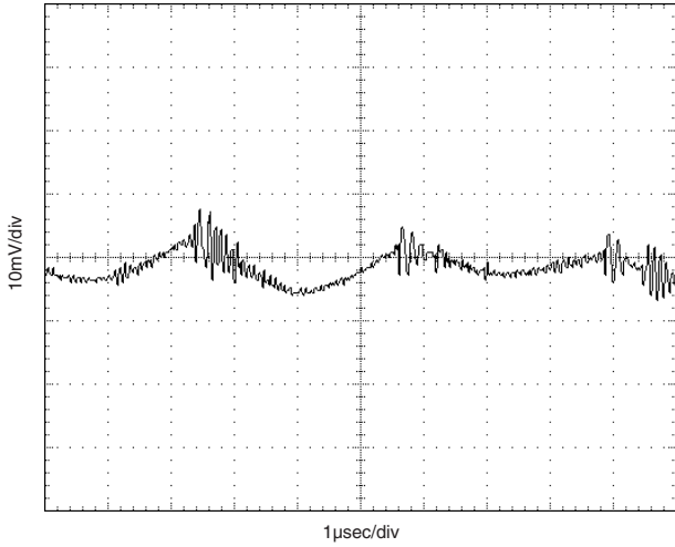
Output Ripple/Noise (VIN = 3.3V, VOUT = 2.5V, Full Load, No External Capacitor)
