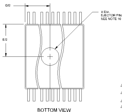
48-Pin Shrink Small Outline Package (SSOP, 300 mils)
