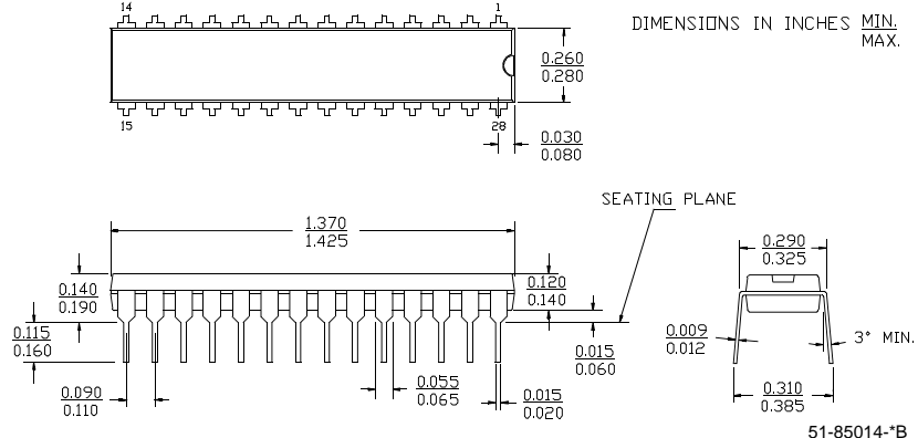
48-lead (600-Mil) Molded DIP P25
