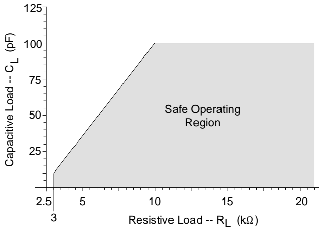
Figure 14. Maximum Loading
